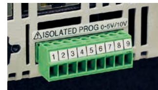
Isolated analog interface (factory option) Voltage control type ISO PROG VOLT CONT PWX OPTION Current control type ISO PROG CURR CONT PWX OPTION
