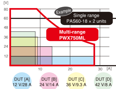
In case of testing four different rating DUTs
